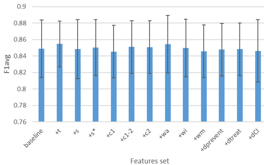
Fig. 8 Histograms that represent the average F1 score (y-axis) and standard deviations under logistic regression for most of the vector sets considered in Table 7 (x-axis)
