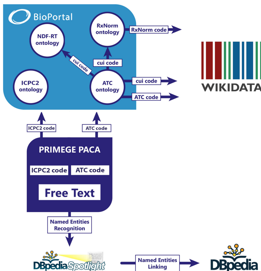
Fig. 6 Workflow to link ATC codes, ICPC-2 codes and named entities in the EMRs with medical domain ontologies and with the knowledge graphs Wikidata and DBpedia
