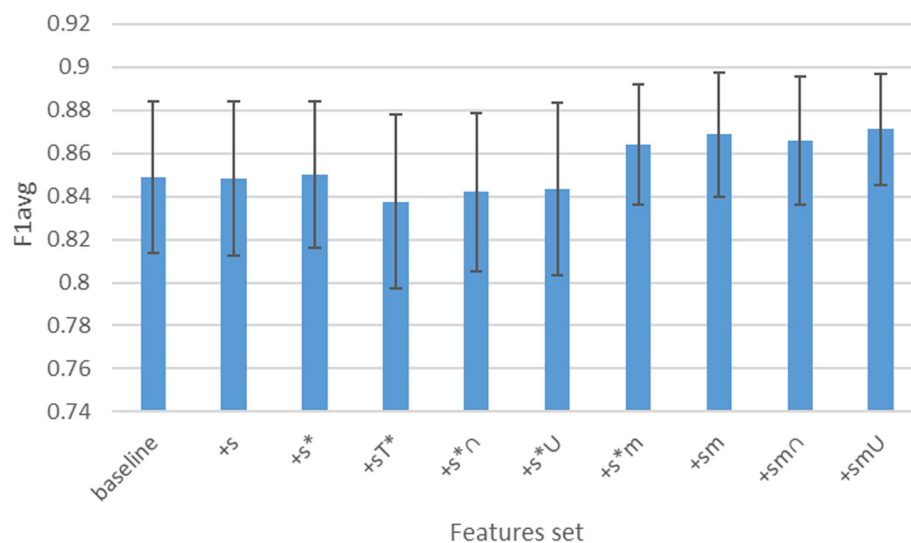
Fig. 9 Histograms that represent the average F1 score (y-axis) and standard deviations under logistic regression for the vector sets considered in Table 7 (x-axis)
