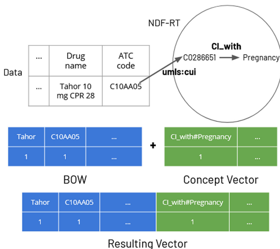
Fig. 5 Concatenation of a bag-of-words representation V and a bag-of-concepts representation C of EMRs. In this example, we use the drug tahor whose main molecule is atorvastatin and we show how we extract and use one of these contraindicated effects (property CI_with ) from the NDF-RT ontology
